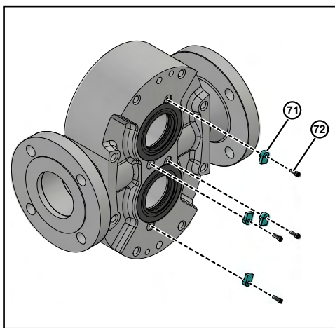
Figure 91 - Install Screws and Retainer-tab
