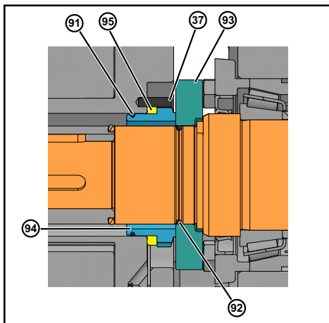
Figure 70 - Single Mechanical Seal
