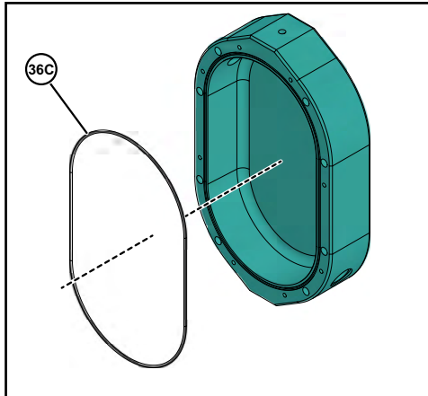
Figure 83 - Install Gasket
