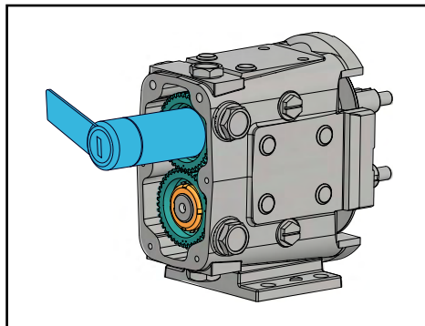
Figure 64 - Install Gear Locknuts
