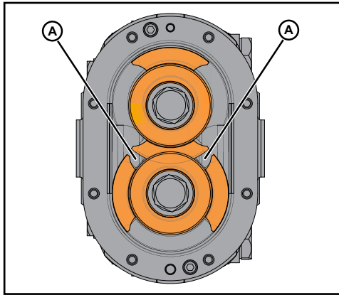
Figure 28 - Rotor to Rotor Tip Clearance
