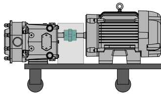
Figure 3 - Portable Base
